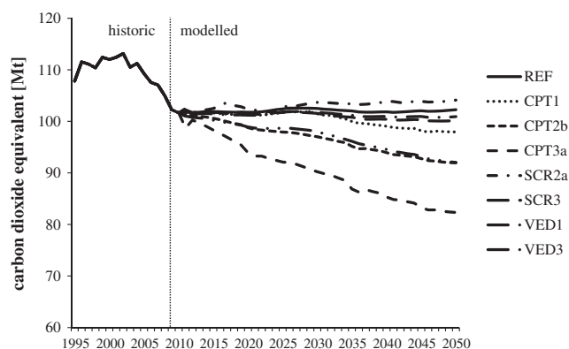
Fig. 7. Life cycle greenhouse gas emissions (as CO 2 e) from cars for a selection of scenarios against the reference case.
