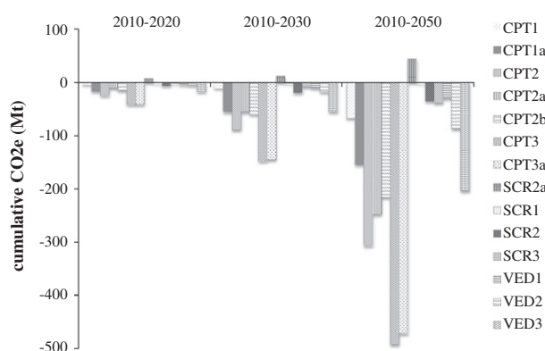
Fig. 8. Life cycle GHG emissions, cumulative savings over baseline (REF) in MtCO 2 e.
