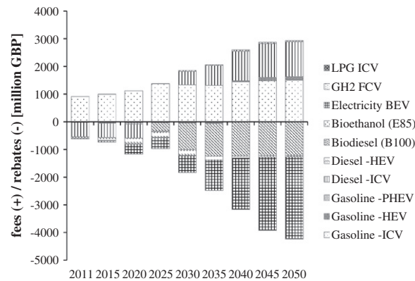
Fig. 10. Revenue streams from fees and rebates for the 'medium' ambition car purchase feebate (CPT2b, with GBP3000 top rebate and GBP0.06/kWh electric fuel duty).
